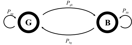
Fig. 2. Gilbert error model state diagram.
