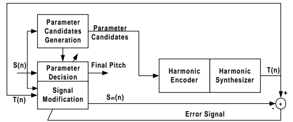
Figure 1: Analysis-by-synthesis parameter estimation in harmonic coding
